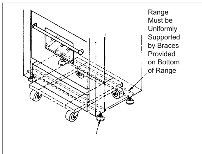
Figure 6: Dolly Positioning
