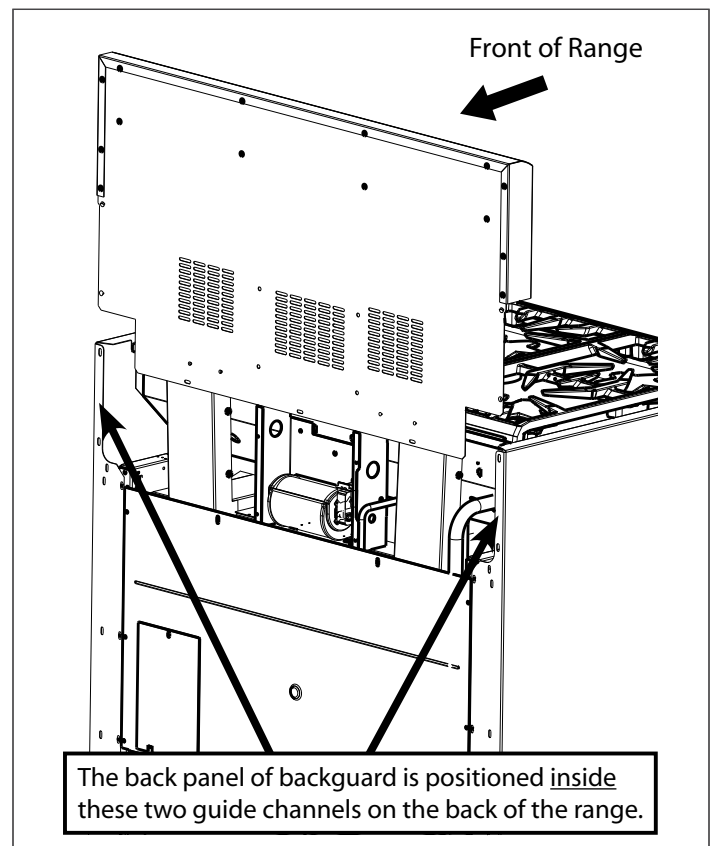
Figure 11: Backguard Installation
