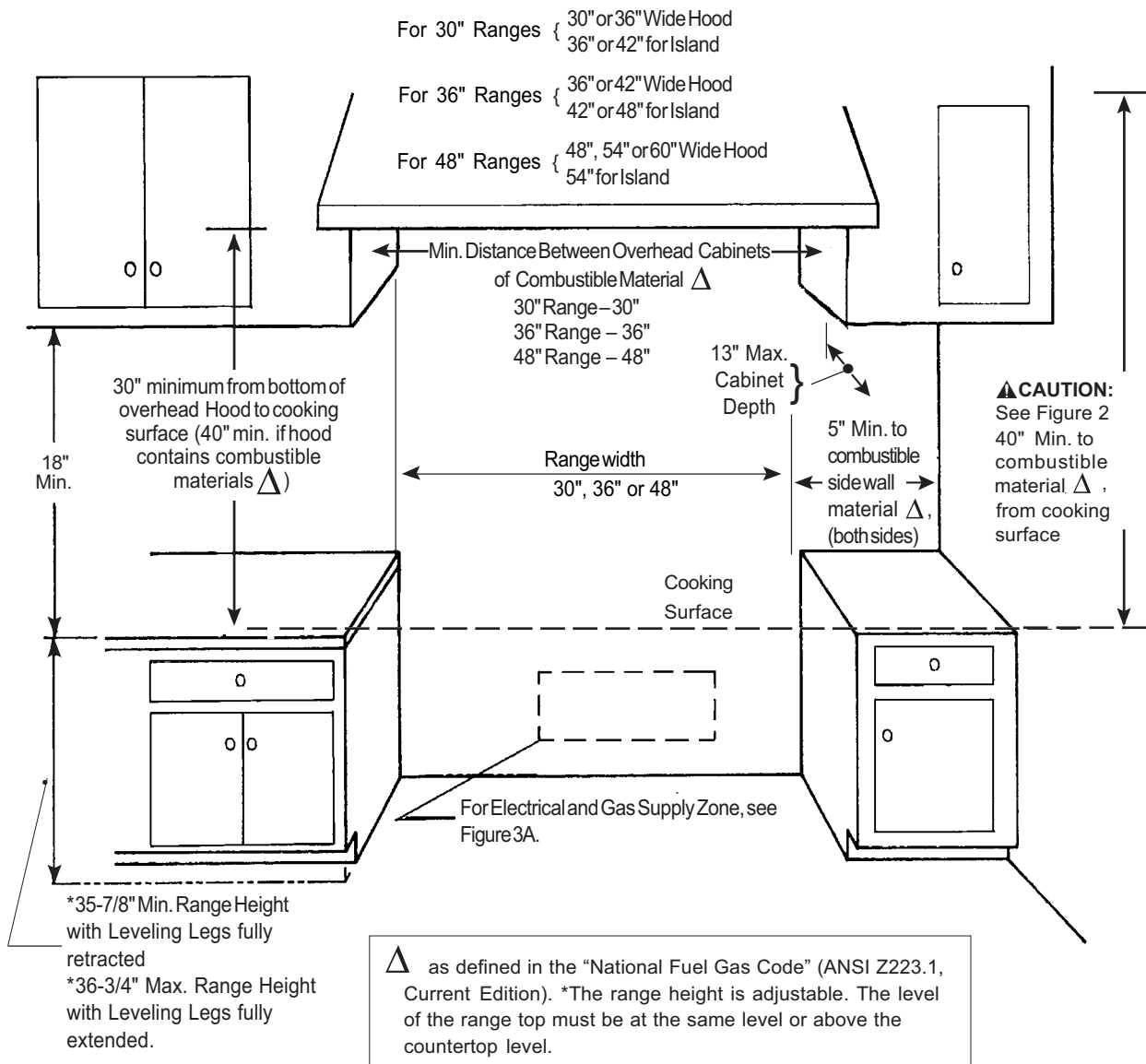
Figure 1: Cabinet Clearances
