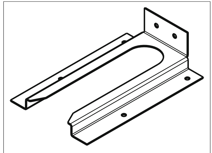
Figure 7: Anti-tip Bracket
