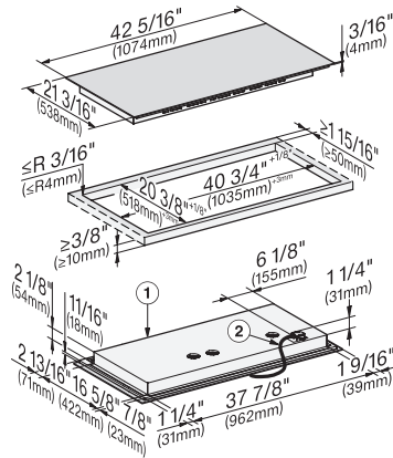
KM7755FL – frameless overlaying installation (*footnote) – drawing
