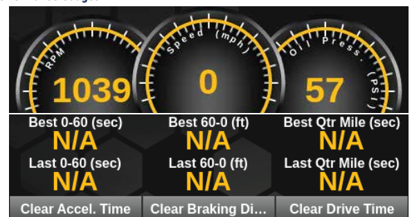
Vehicle Information
