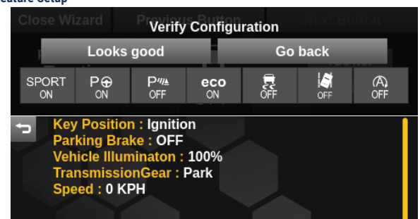
Feature Setup
