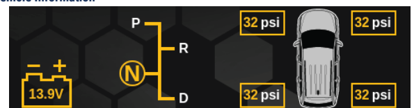
Feature Setup
