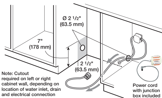
Example of Hardwire Installation
