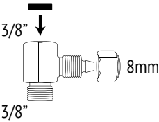
Hot Water T-adapter (3/8" x 3/8" x 8mm)
