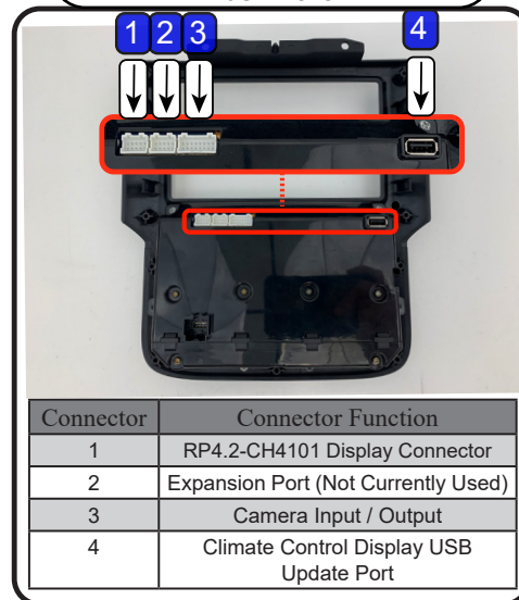
Fig.1: Rear of RPK4-CH4101 Radio Dash Bezel
