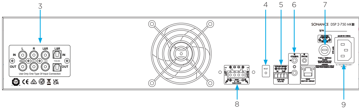
Figure 4: DSP 2-750 MKIII Two-Channel Power Amplifier Rear Panel
