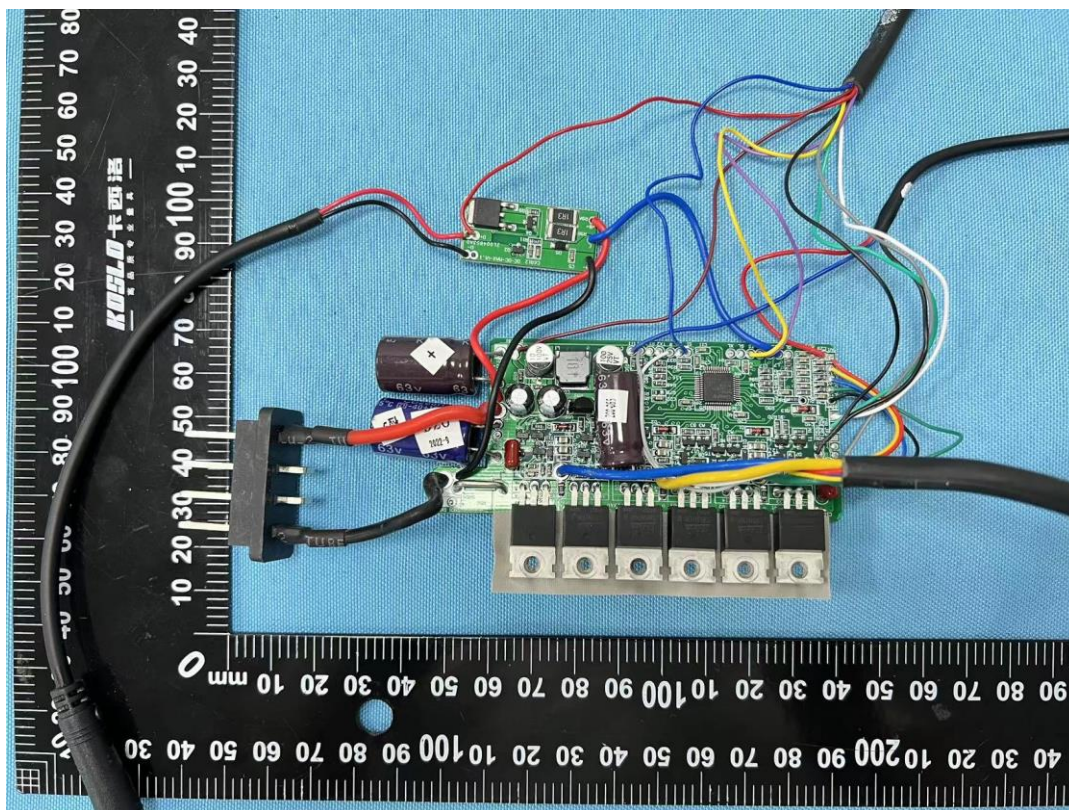
Figure 14.: Controller view
