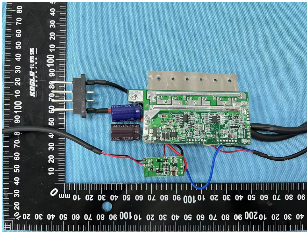
Figure 15.: Controller view
