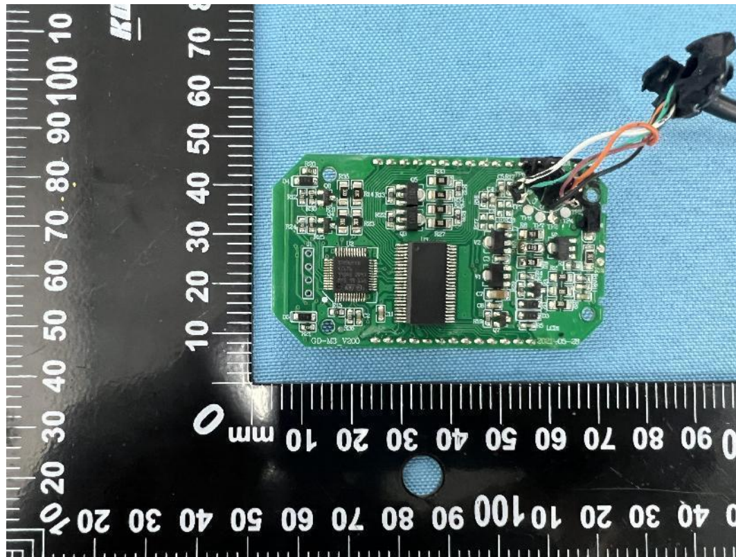
Figure 19.: Dashboard internal view
