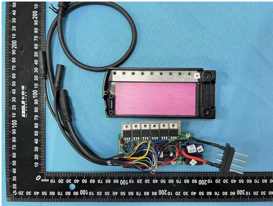
Figure 13.: Controller view
