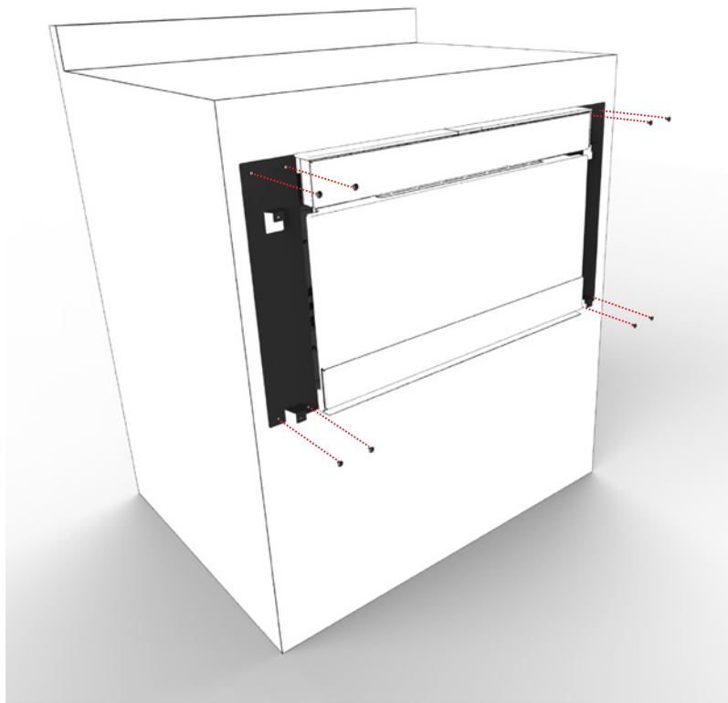
3. Install SKMD30E3DS brackets
