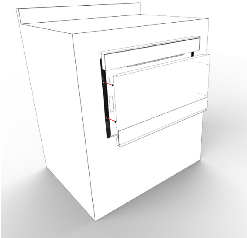
2. Install SMD2480CS Microwave Drawer
