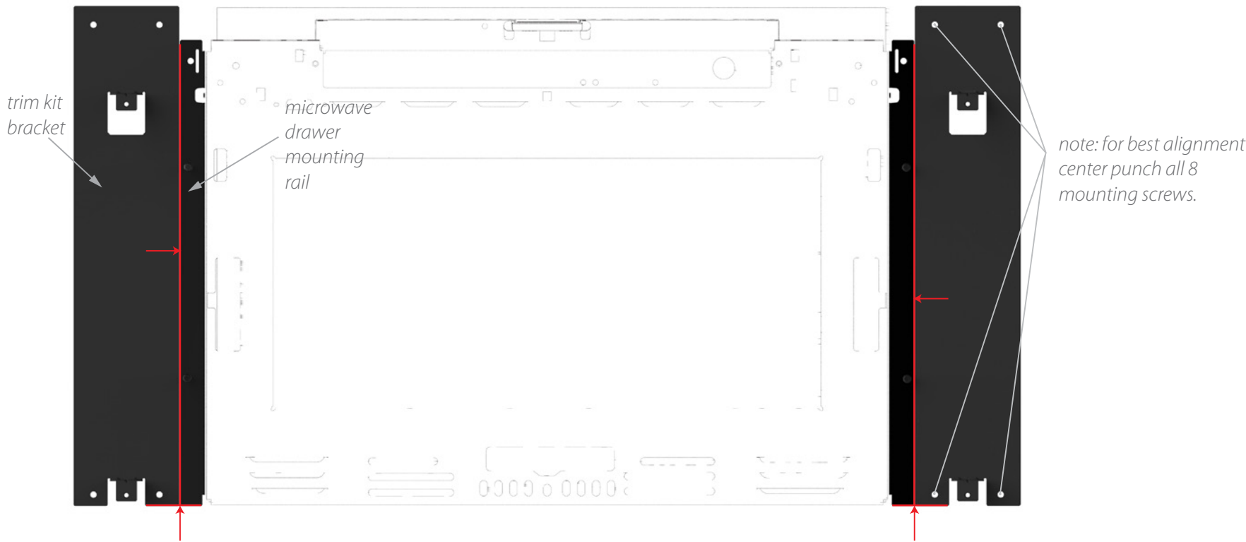
3a. Align the Bottom and Sides of trim kit brackets with Microwave Drawer mounting rails:
