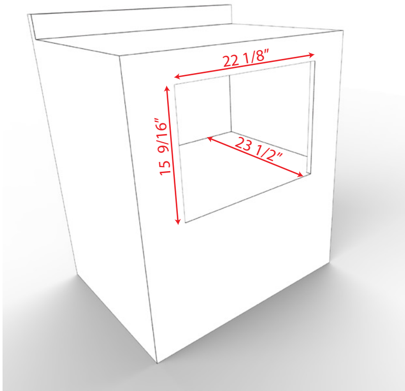
1. Cabinet Cutout: W 22 1/8" x H 15 9/16" x D 23 1/2"
