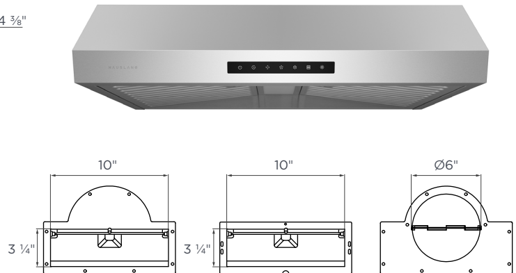
TOP RECTANGULAR EXHAUST ADAPTER
