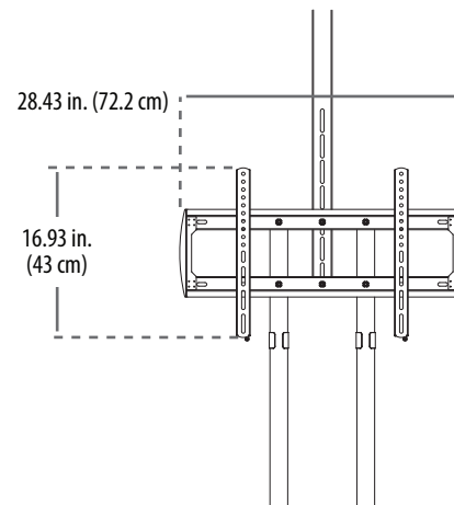
TV MOUNTING PLATE
