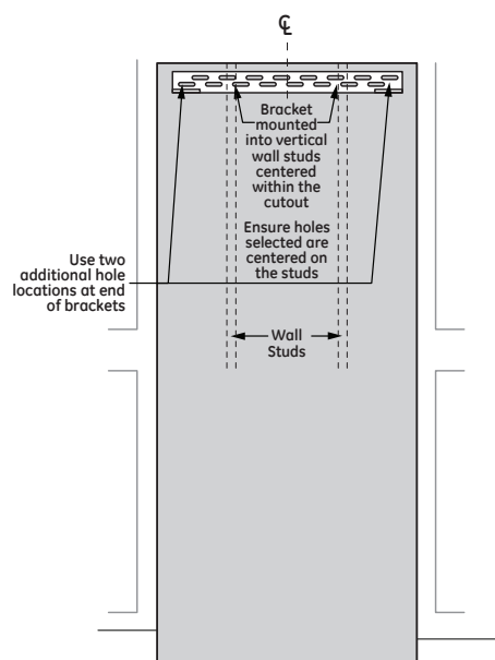
FRONT VIEW OF CUTOUT WITH ANTI-TIP BRACKET
