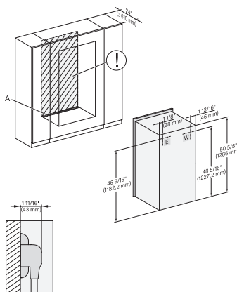
H 6x80 BP2, H 6x80-2BP2, H7x80BP2wide front installation, installation drawing, Proud, NA
