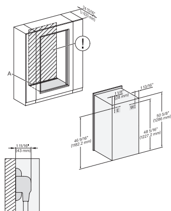
H 6x80 BP2, H 6x80-2BP2, H7x80BP2, wide front installation, installation drawing, Flush inset, NA
