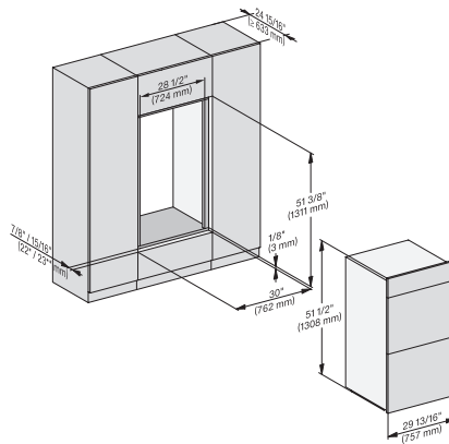
H 6x80 BP2, H 6x80-2BP2, H 7xxx fitting, installation drawing, Flush inset, NA
