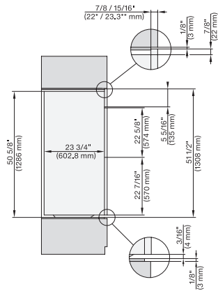
H 6x80 BP2, H 6x80-2BP2, H 7x8x, side view, installation drawing, Flush inset, NA
