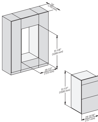
H 6x80 BP2, H 6x80-2BP2, H7x80BP2, fitting, installation drawing, Proud, NA
