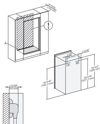
H 6x80 BP2, H 6x80-2BP2, H7x80BP2, installation, installation drawing, Flush inset, NA
