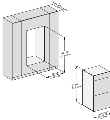
H 6x80 BP2, H 6x80-2BP2, H7x80BP2, fitting wide front, installation drawing, Proud, NA
