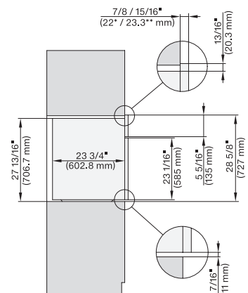
H 6x8x BP, H 6x80-2BP, H2x80BP, H7x8xBP(X), side view, installation drawing, Proud, NA
