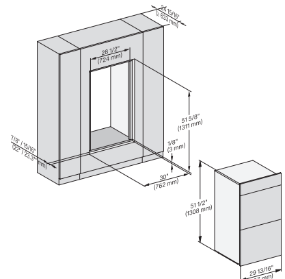
H 6x80 BP2, H 6x80-2BP2, H7xxx fitting wide front, installation drawing, Flush inset, NA
