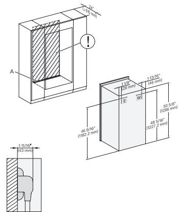
H 6x80 BP2, H 6x80-2BP2, H7x80BP2, installation, installation drawing, Proud, NA
