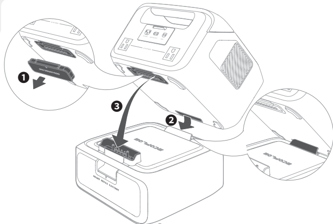
EcoFlow RIVER 3 Plus Smart Extra Battery
