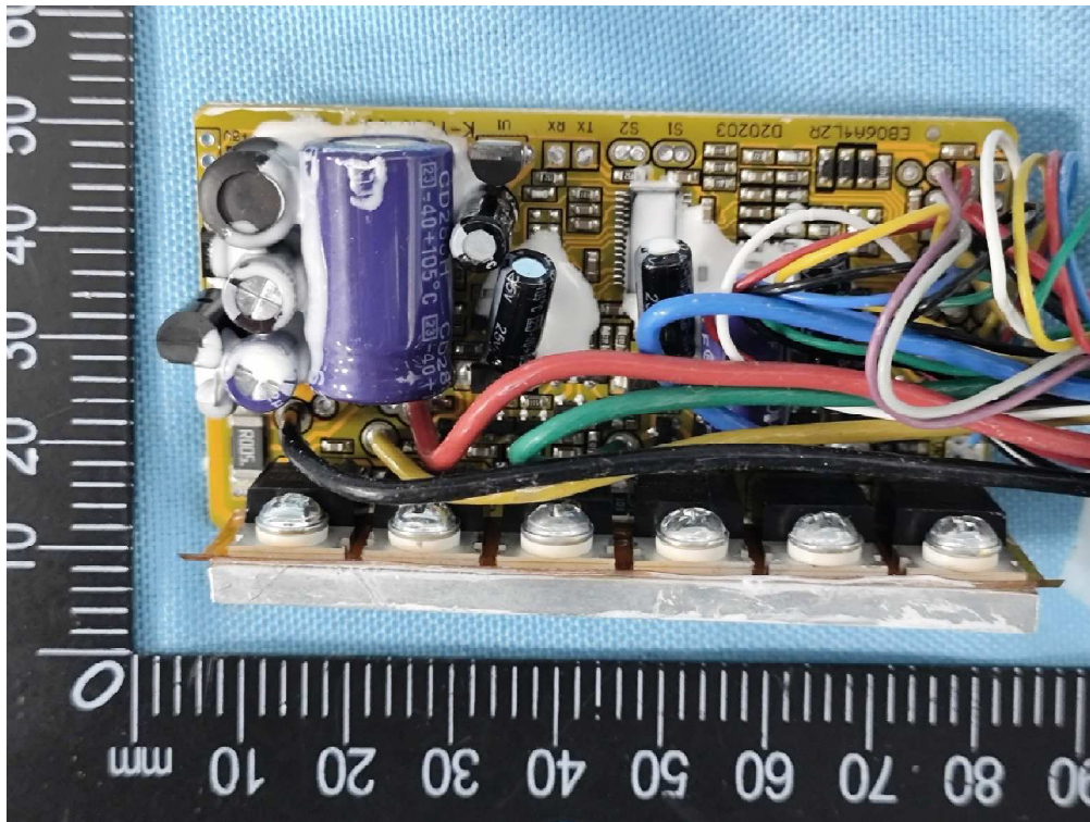
Figure 15.: Controller PCB top view
