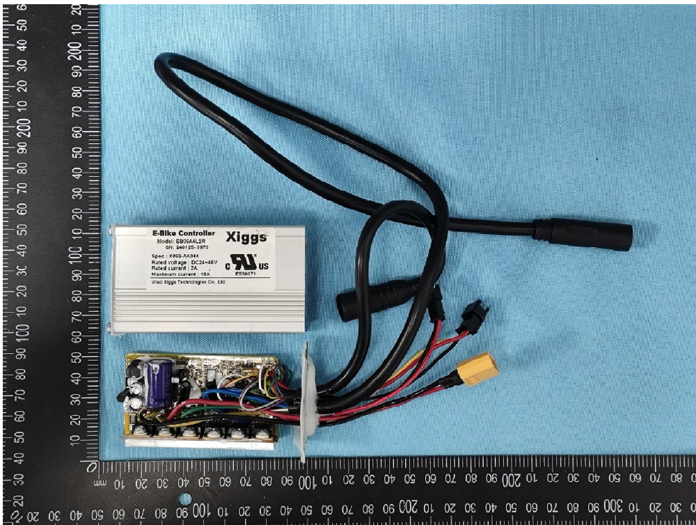
Figure 14.: Controller view
