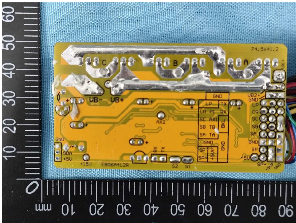
Figure 16.: Controller PCB bottom view
