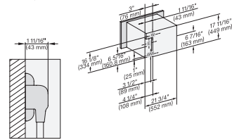
installation 30 inch Proud wide front DGC30 XL, installation drawing, NA
