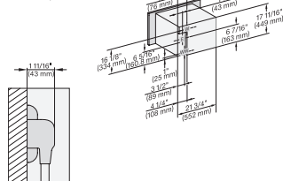
installation 30 inch Flush inset wide front DGC30 XL, installation drawing, NA
