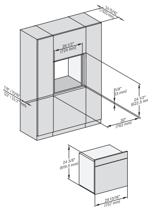
Installation 30 inch Flush inset DGC30 XXL, installation drawing, NA
