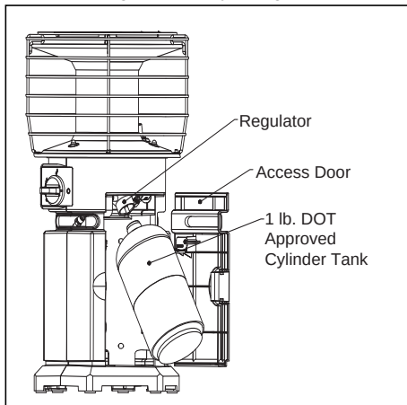
Fig. 1 - 1 lb. Cylinder Tank Installation
