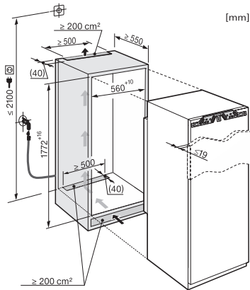
FNS37492iDE (installation drawings)
