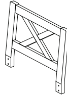
Backrest of chair /Dossier de la chaise D x 8
