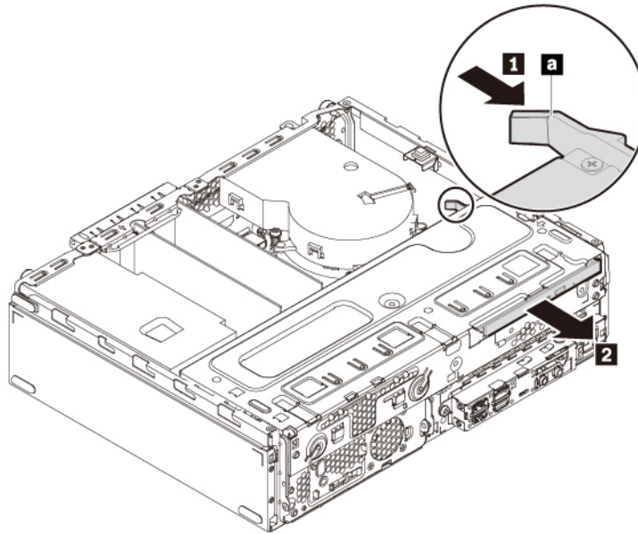
Figure 33. Removing the slim optical drive
