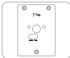
c.Mounting Plate
