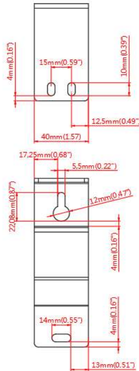
Wall/Ceiling Installation Bracket Dims
