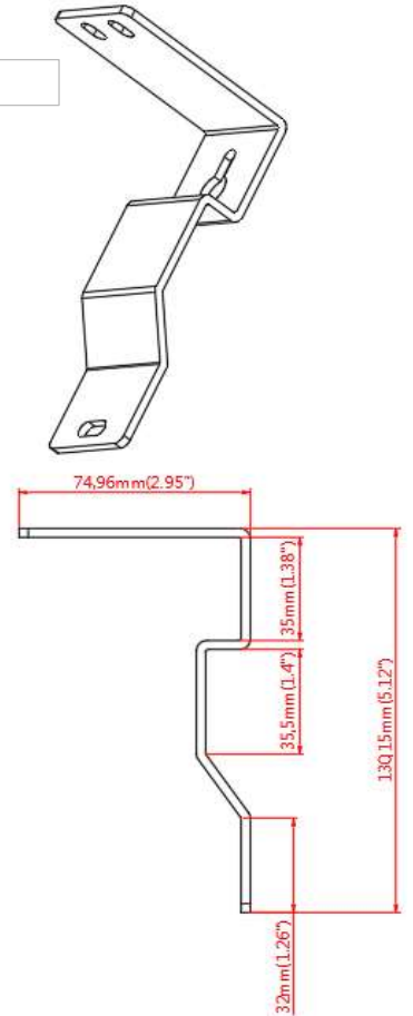
Wall/Ceiling Installation Bracket Dims
