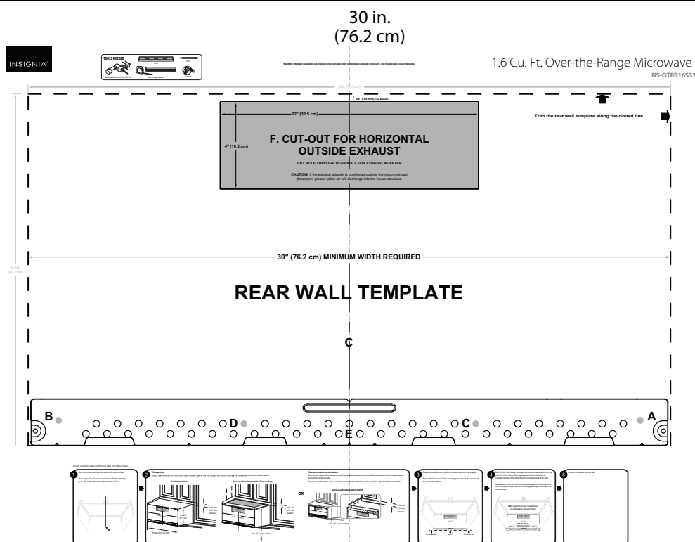
Rear wall template
