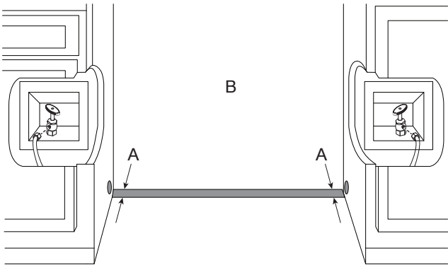
A. 1/2" (13 mm) B. Waterline access hole to be within 1/2" (13 mm) from back wall.
