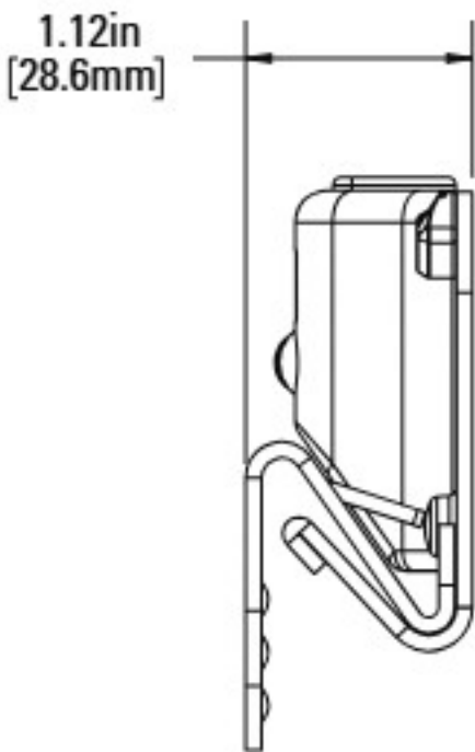
END VIEW
