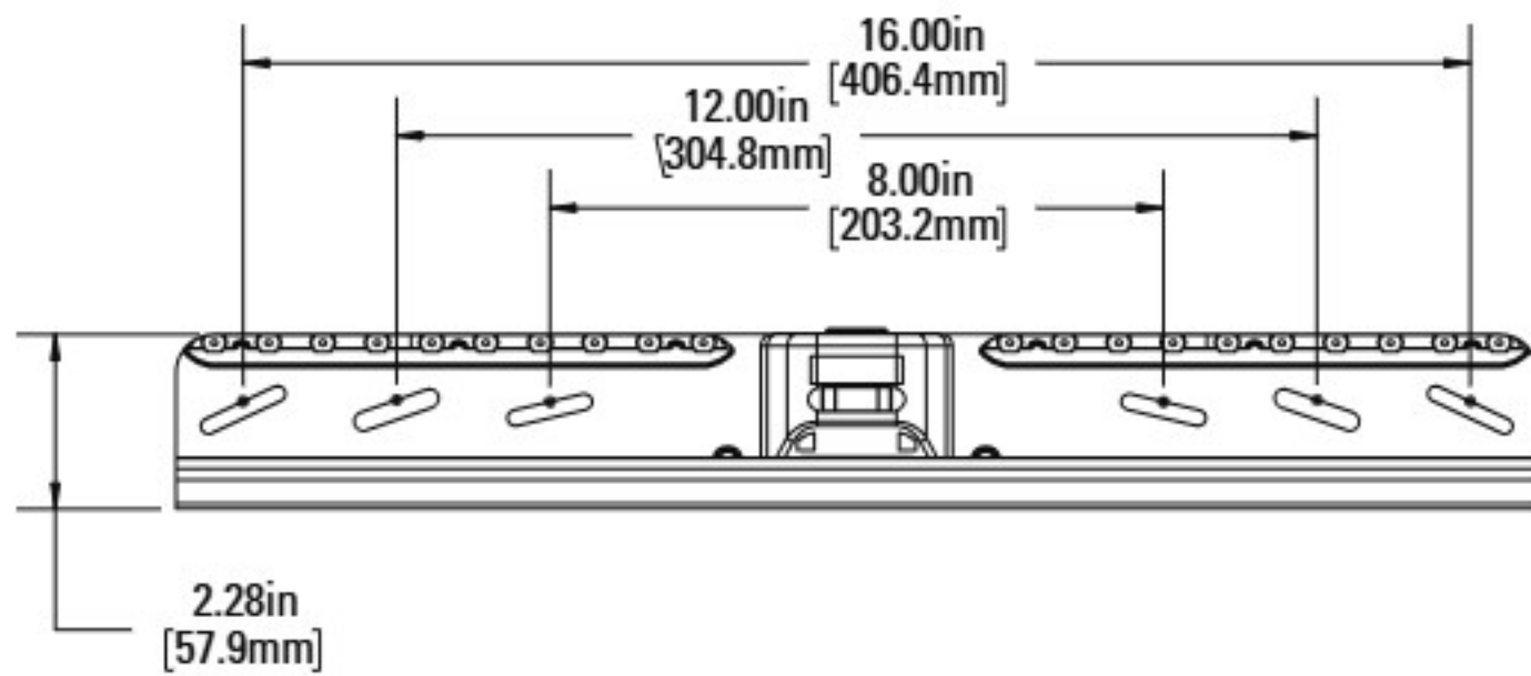
WALL PLATE
