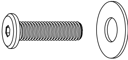
ALLEN KEY BOLT: M8 X 30 mm - QTY 14 WASHER: \varnothing 19/\varnothing 12 X 1 mm - QTY 14 QTY 14 SETS
